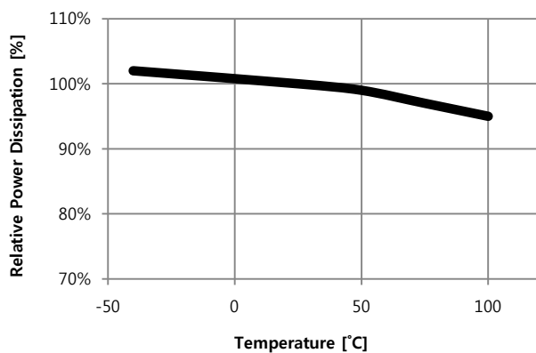
7-3 Temperature Characteristics
