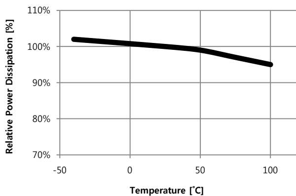
7-3 Temperature Characteristics
